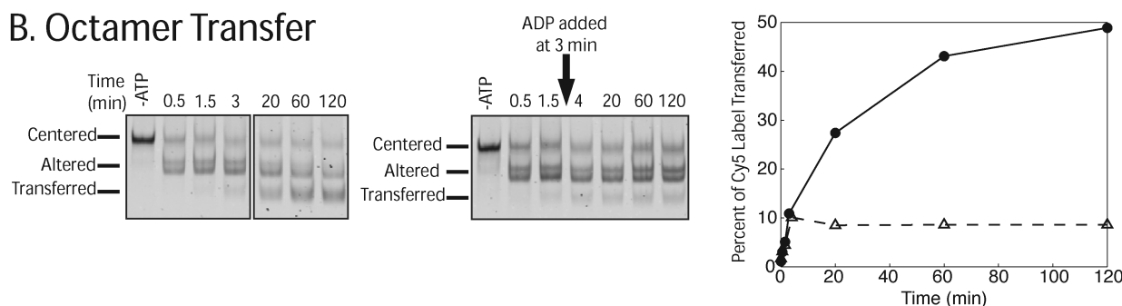
FIGURE 4: Continuous RSC activity is necessary for formation of a stable transfer product. Dimer transfer reactions (A) and octamer transfer reactions (B) using the substrates from Figure 1 at 1 mM ATP were analyzed on a native gel. The left gels show the reaction with no ADP added, and the right gels show reactions in which excess ADP was added after 3 min. The gels were scanned in the Cy5 channel. The graph shows the quantification of transfer for the reactions with no ADP added as black circles with a solid black line and ADP added at 3 min as open triangles with a dashed line. In (A) the values for dimer transfer are calculated from three independent experiments; error bars show the standard error of the mean. For octamer transfer one representative experiment is shown. Other experiments where ADP was added at different time points showed the same requirement for ATP (data not shown). In (B), left panel, all of the time points shown are from the same gel, but lanes between the 3 and 20 min time points were omitted to enable a direct visual comparison with the gel in the right panel.
